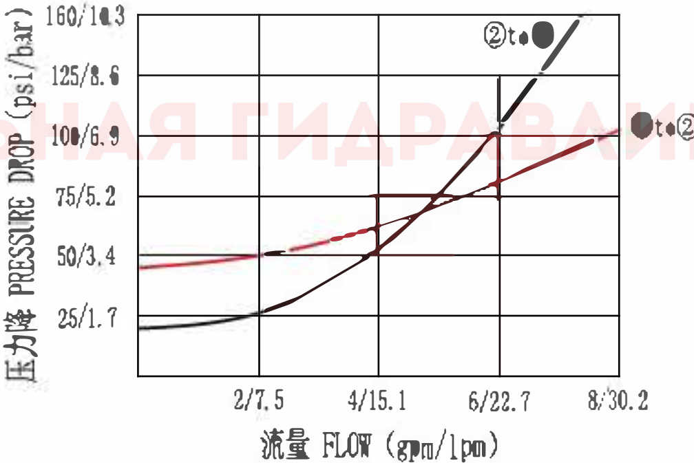
压力-流量曲线 PRESSURE DROP VS. FLOW 32cSt oil @ 40° C
